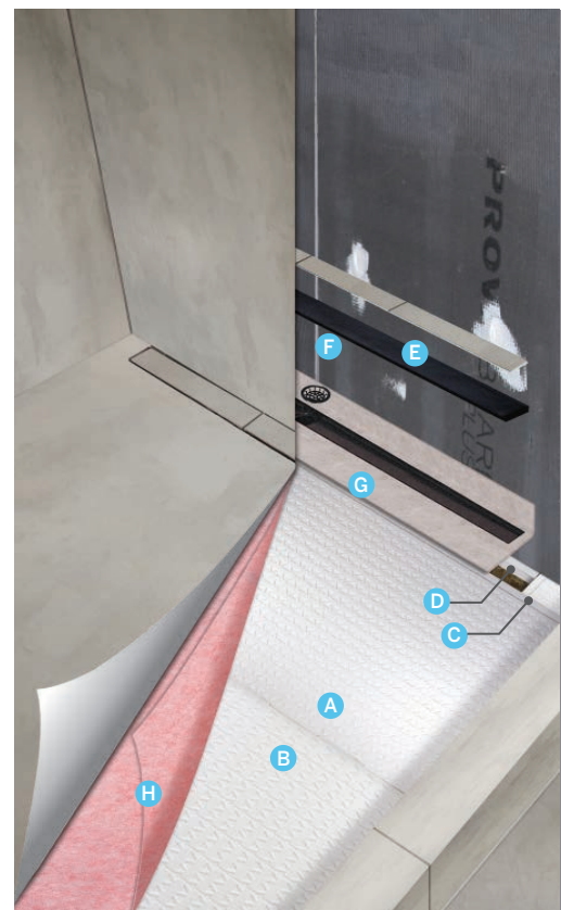
END DRAIN WITH PROVA LINEAR PAN EXTENSION® KIT - 4' X 6' (122 cm x 183 cm)
