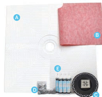
48" x 48" (122 cm x 122 cm) Kit with ABS Drain, Center Placement
