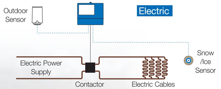
ProMelt Smart Controller
